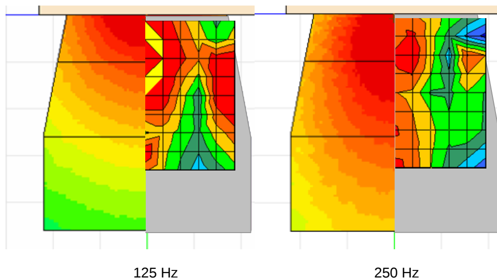
Figure 4: Sound pressure distributions by frequency band (low frequency bands) (left diagram: the results of Y-S 3 , right diagram: measured results)
