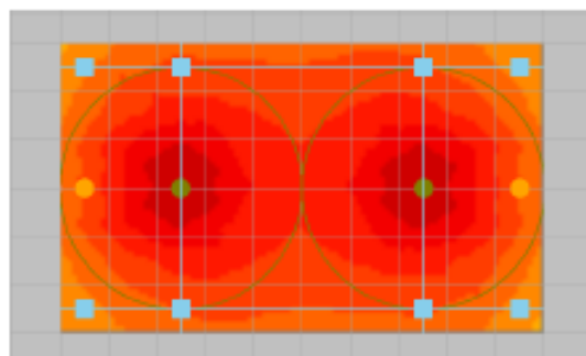
SPL Map[ HIGH, 2kHz - 8kHz ]
